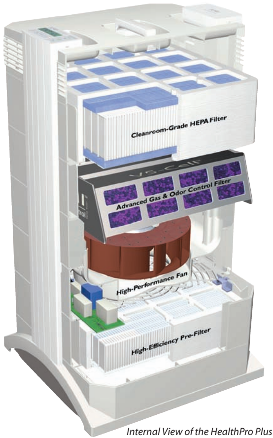
Internal View of the HealthPro Plus
